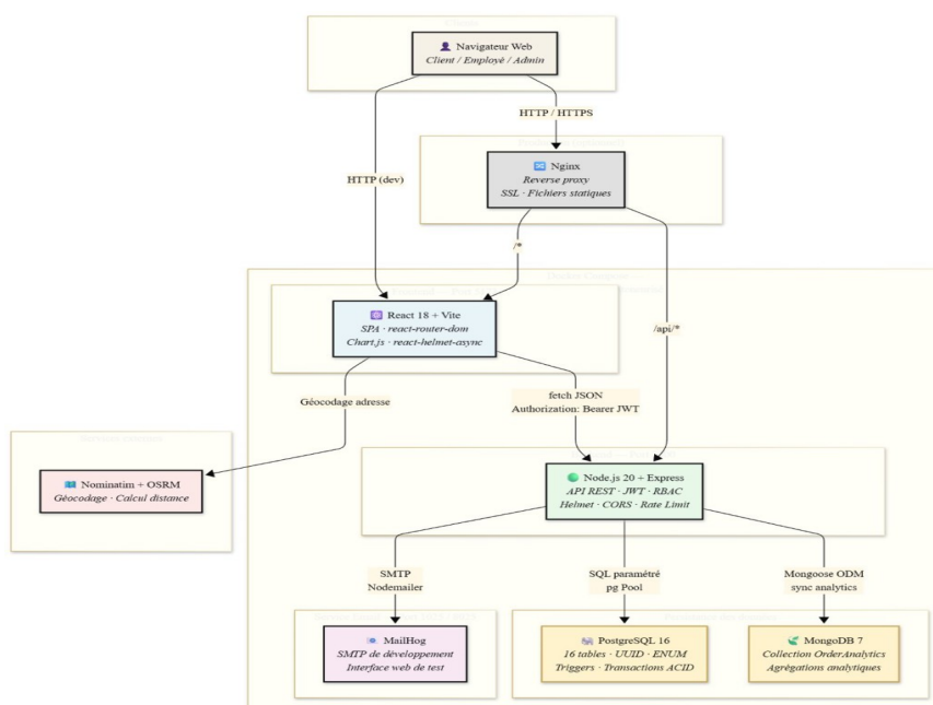
Figure 1 — Architecture générale de l'application
